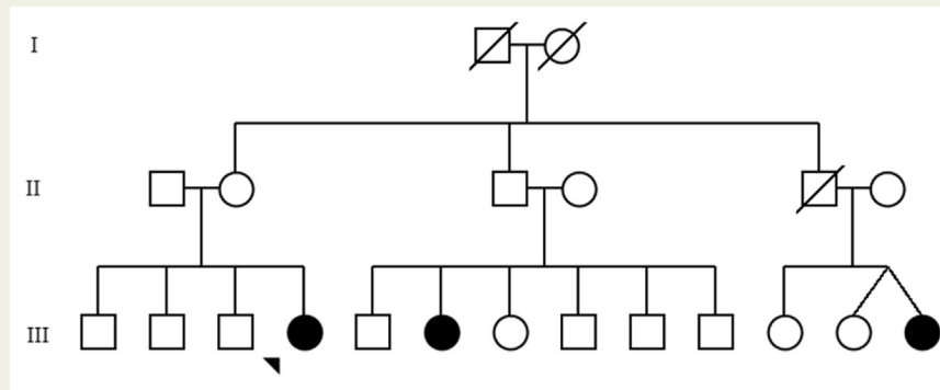
Figure 3 Pedigree of a family in which three first cousins (generation III) had a spontaneous coronary artery dissection (SCAD) episode at age 40 (propositus; indicated by the arrowhead), 51 and 37 years.
